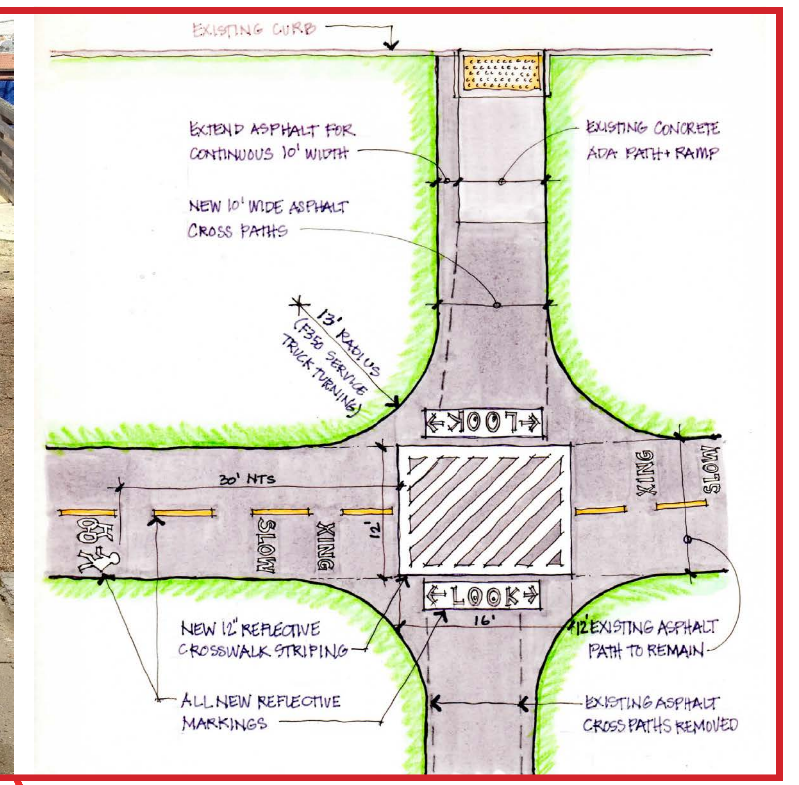
Concept for Typical Intersection Striping
